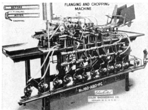
The Eisler syringe flange chopper, 1943. (Patent No. 2,445,000.)
